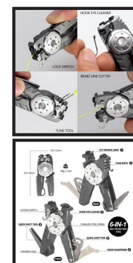
6-IN-1 TOOL
